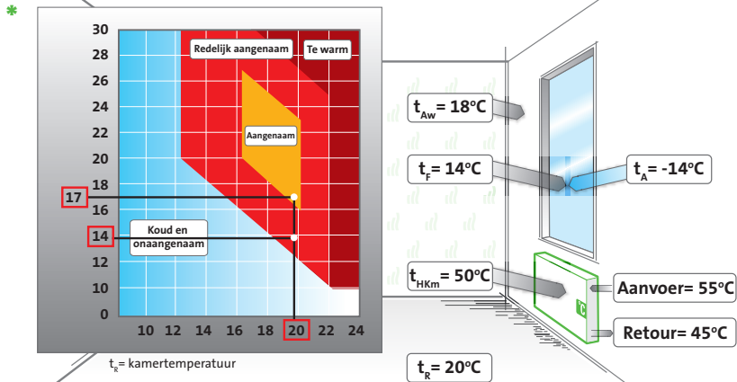
Afb. 2.4 EnEV 2002 (55°/45°/20°C)
